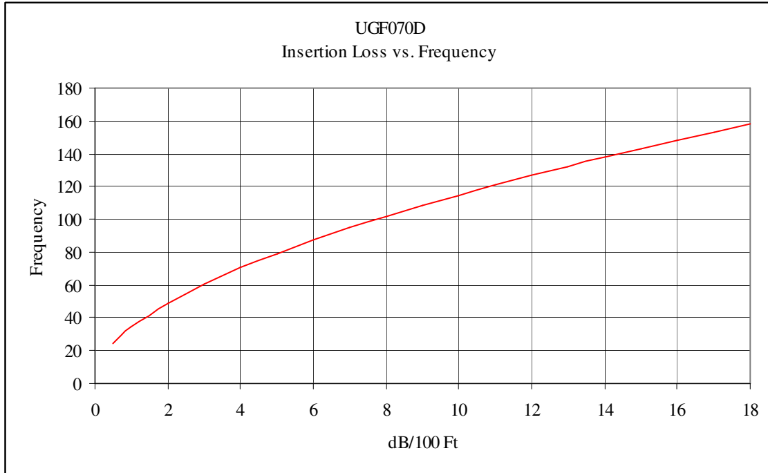
Fig. 4 UGF070D Maximum Insertion Loss
