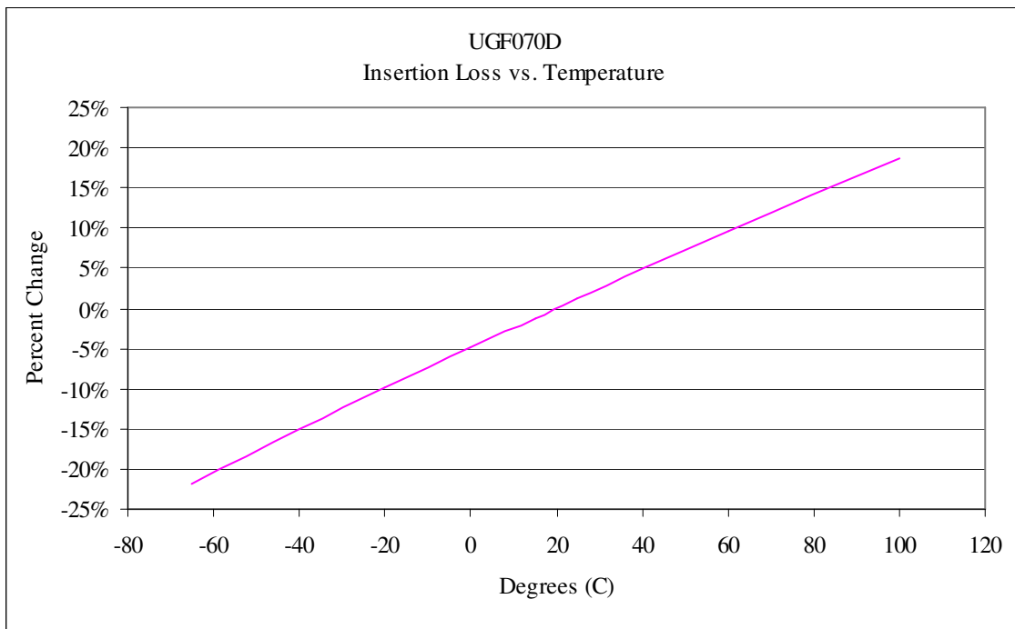
Fig. 5 UGF070D Maximum Insertion Loss Change vs. Temperature
