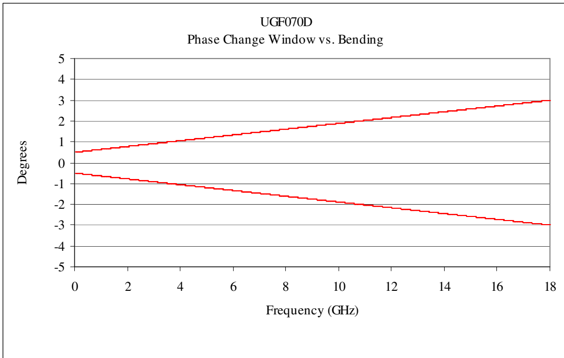
Fig 6 UGF070D Phase Change vs. Bending
