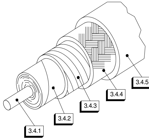
Fig. 1 UGF070D Cable Construction
