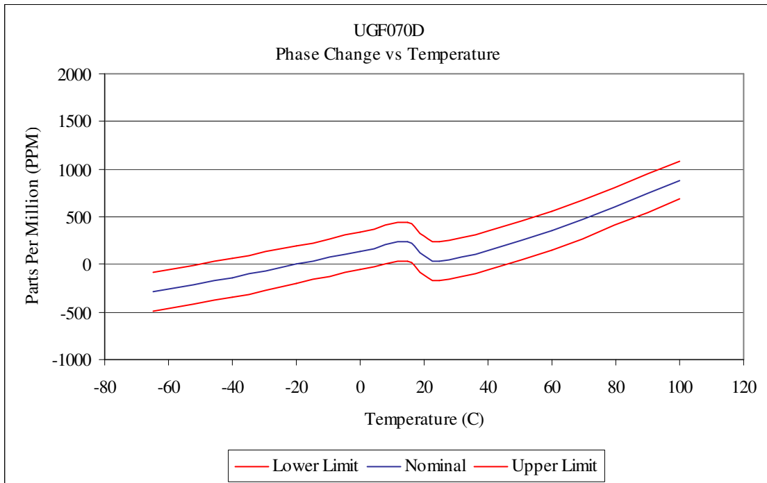
Fig. 7 UGF070D Phase Change vs. Temperature
