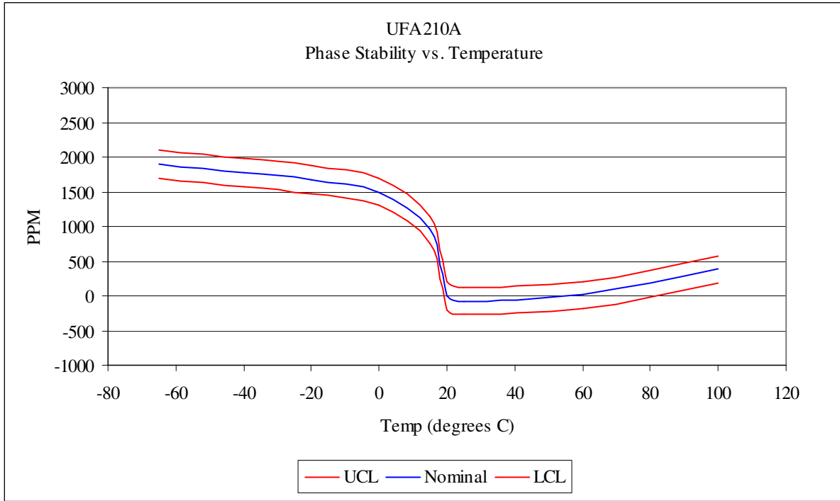
Fig. 7 UFA210A Phase Change vs. Temperature
