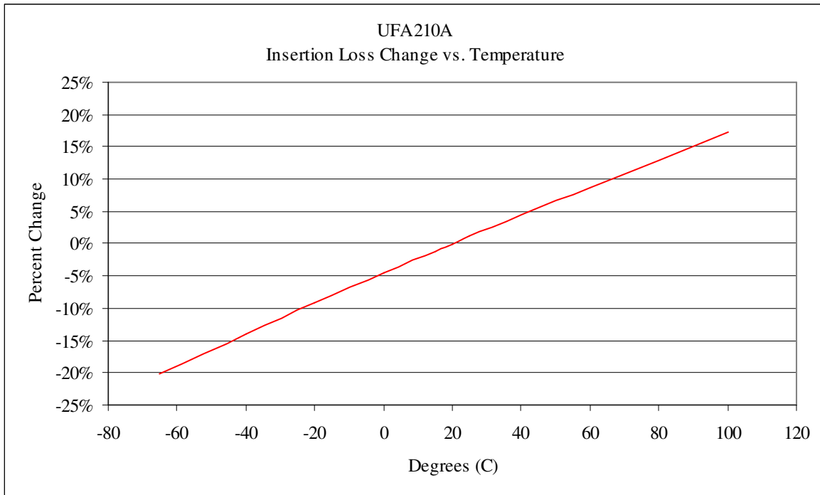
Fig. 5 UFA210A Maximum Insertion Loss vs. Temperature
