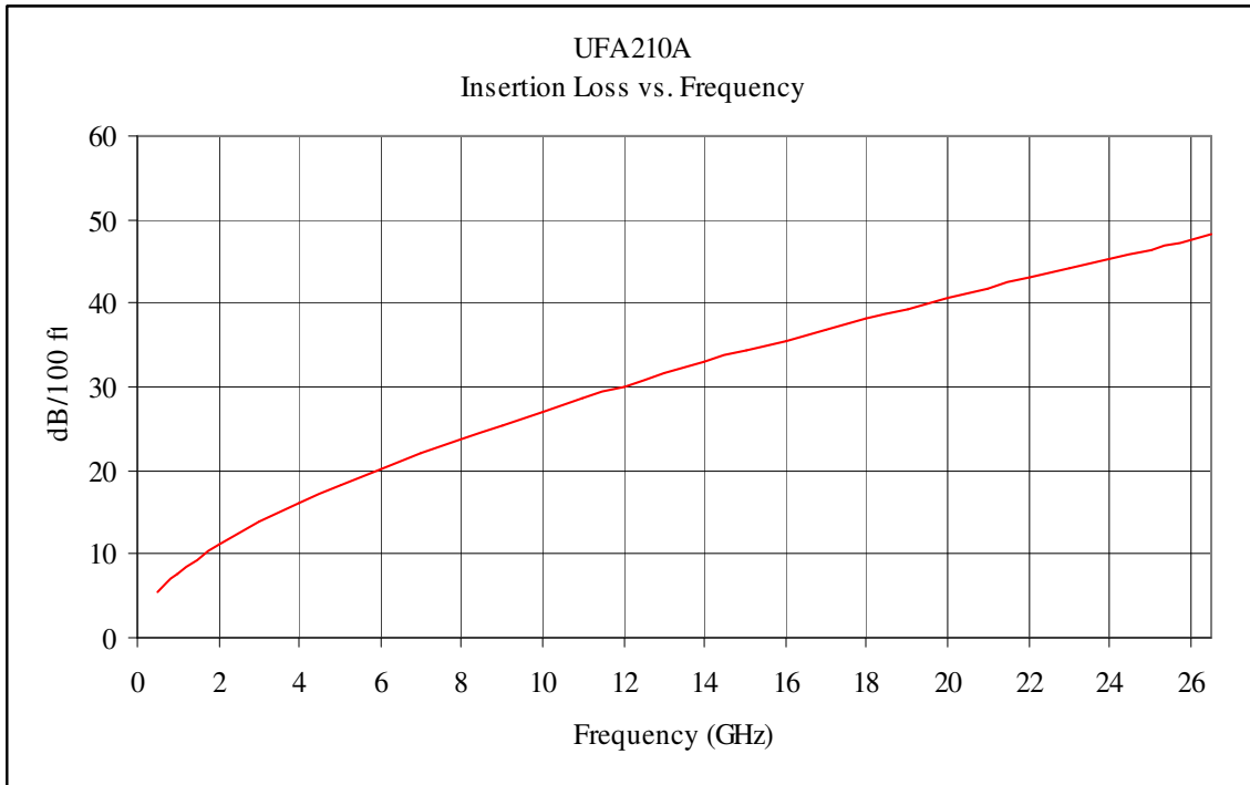
Fig. 4 UFA210A Maximum Insertion Loss
