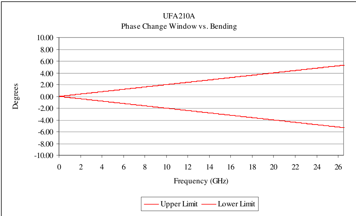
Fig 6 UFA210A Phase Change vs. Bending
