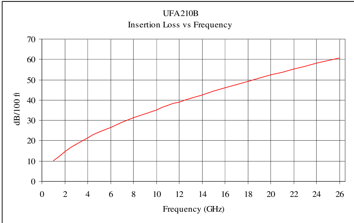
Fig. 4 UFA210B Maximum Insertion Loss
