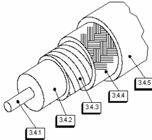
Fig. 1 UFA210B Cable Construction
