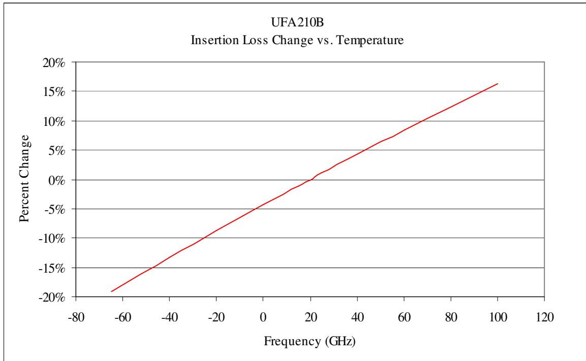
Fig. 5 UFA210B Maximum Insertion Loss vs. Temperature
