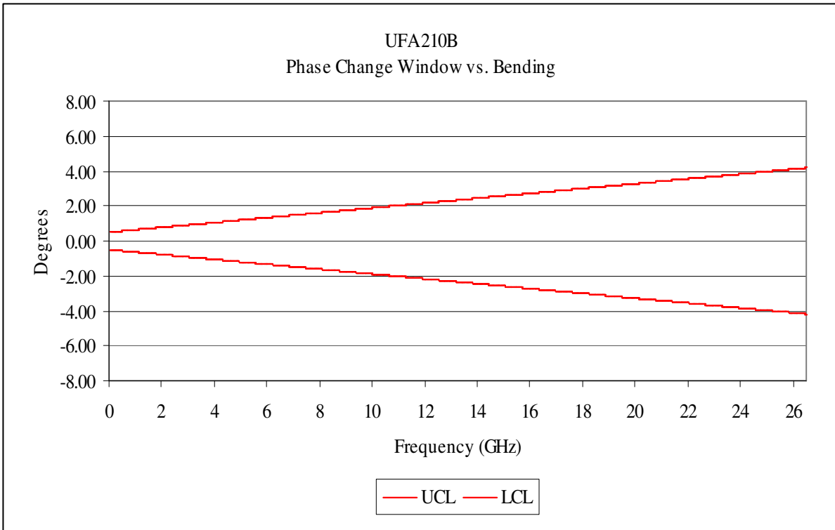
Fig 6 UFA210B Phase Change vs. Bending
