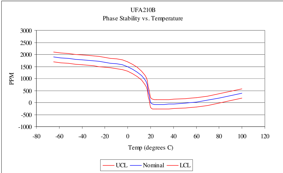
Fig. 7 UFA210B Phase Change vs. Temperature
