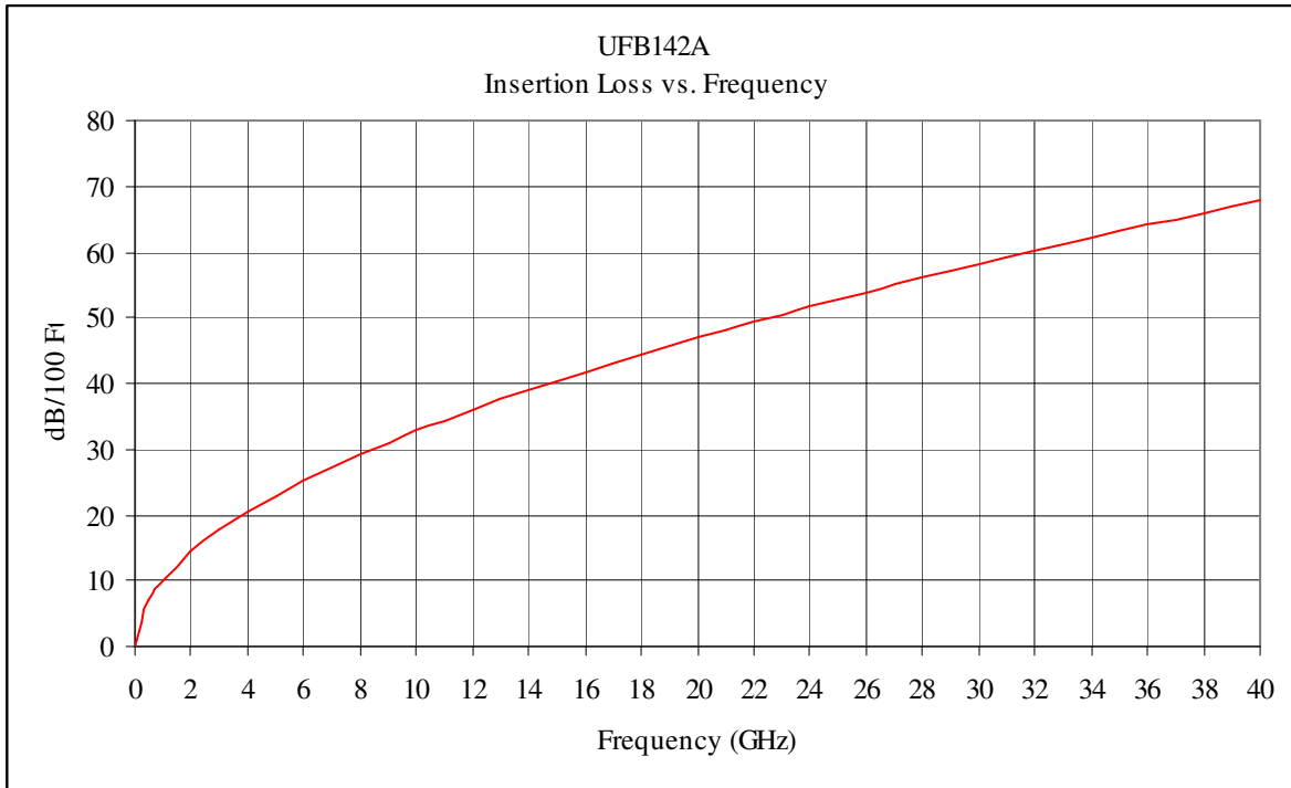
Fig. 4 UFB142A Maximum Insertion Loss
