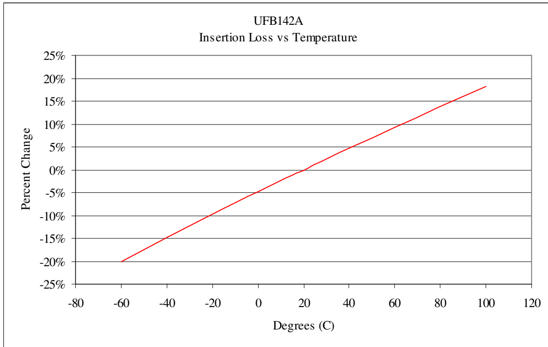
Fig. 5 UFB142A Maximum Insertion Loss Change vs. Temperature
