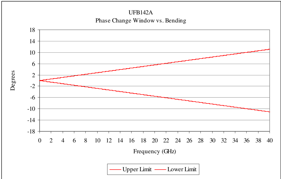
Fig 6 UFB142A Phase Change vs. Bending
