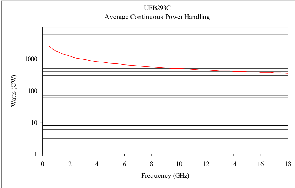
Fig. 8 UFB293C Power
