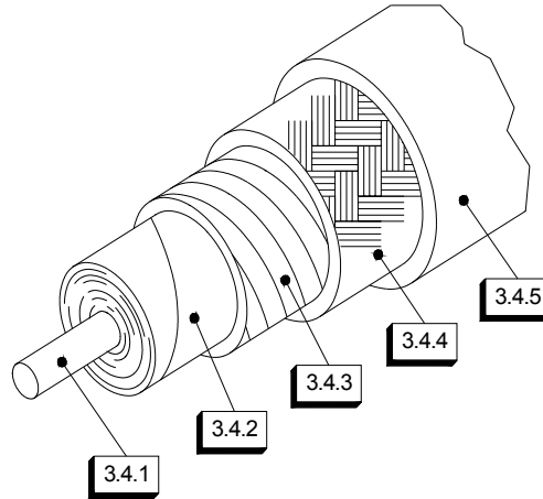
Fig. 1 UFB293C Cable Construction
