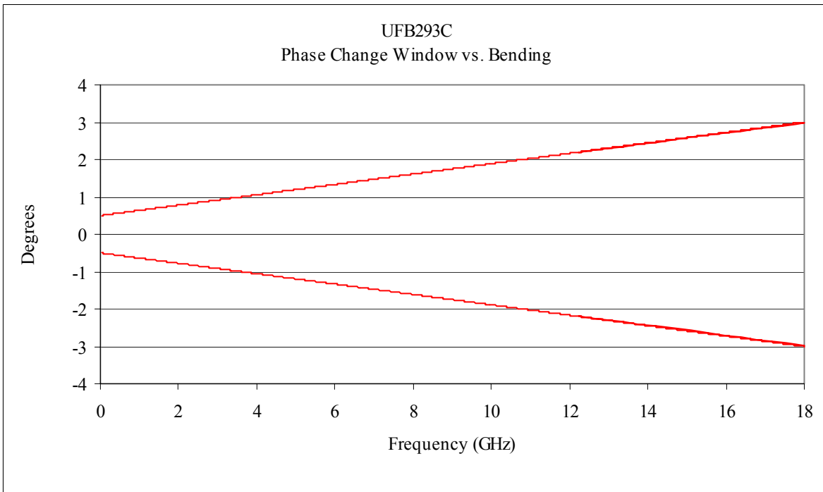
Fig 6 UFB293C Phase Change vs. Bending
