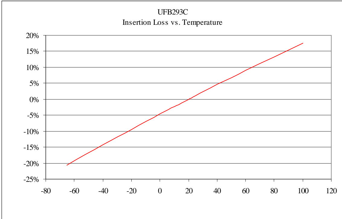
Fig. 5 UFB293C Maximum Insertion Loss vs. Temperature
