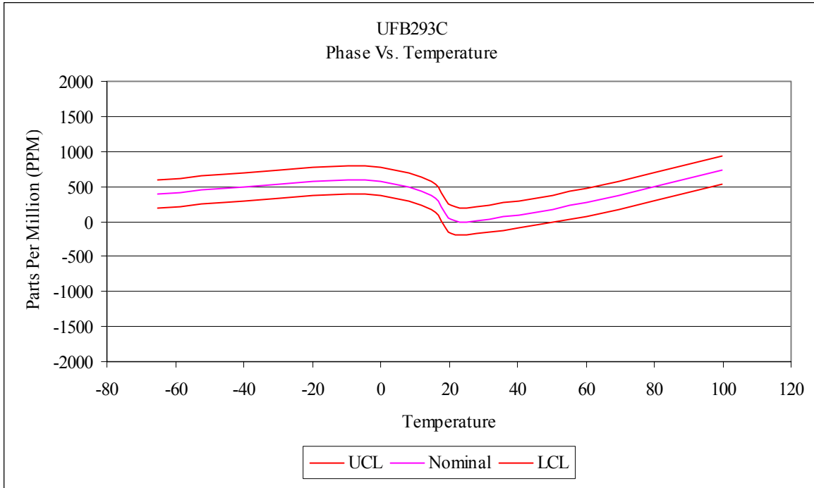
Fig. 7 UFB293C Phase Change vs. Temperature
