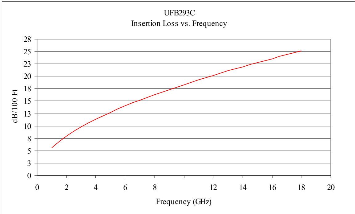
Fig. 4 UFB293C Maximum Insertion Loss
