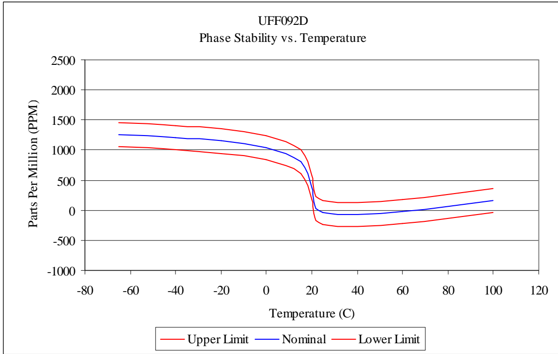
Fig. 7 UFF092D Phase Change vs. Temperature
