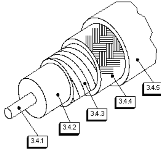
Fig. 1 UFF092D Cable Construction
