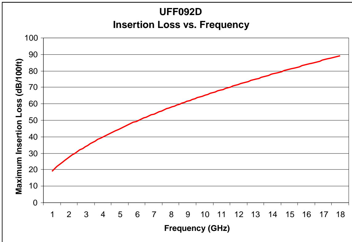
Fig. 4 UFF092D Maximum Insertion Loss
