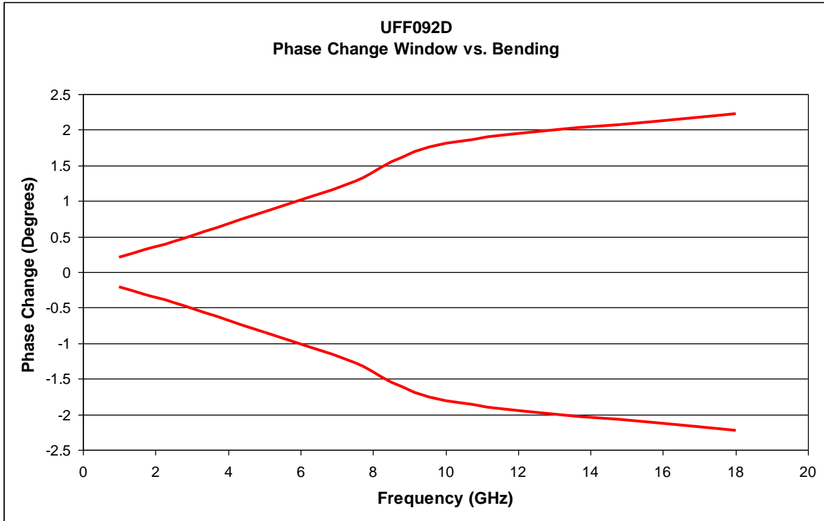
Fig 6 UFF092D Phase Change vs. Bending
