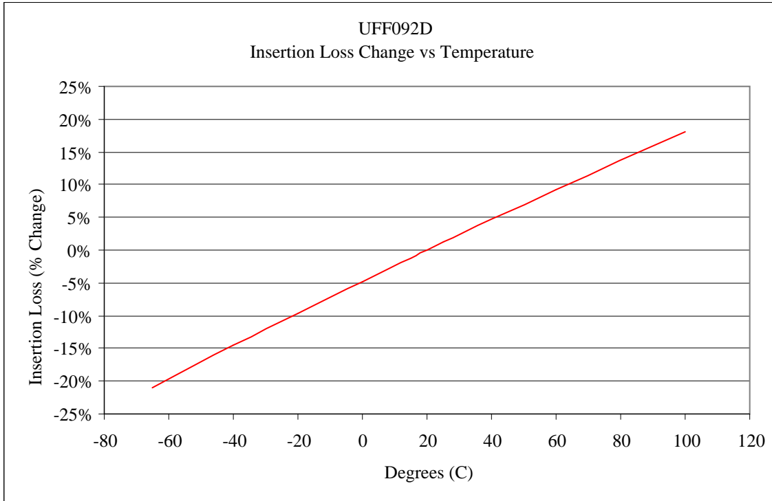
Fig. 5 UFF092D Maximum Insertion Loss Change vs. Temperature
