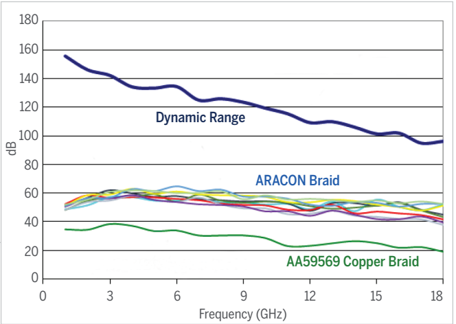
Figure 1: RF Shielding effectiveness of Aracon braid and AA59569 copper braid when tested in a mode-stirred chamber per IEC 61000-4-21, Annex F.
