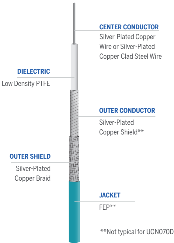
Figure I. Typical microwave cable construction
