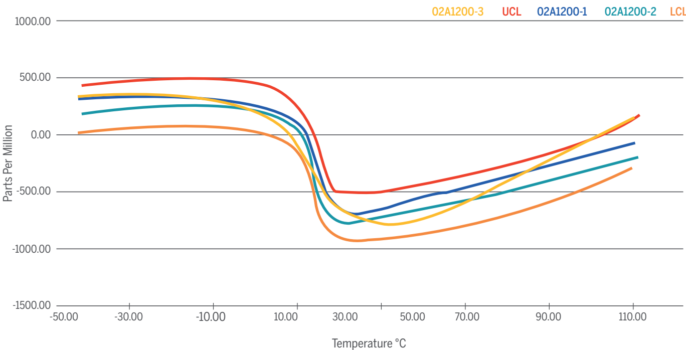
Figure II. Phase Change versus Temperature for UFB311A
